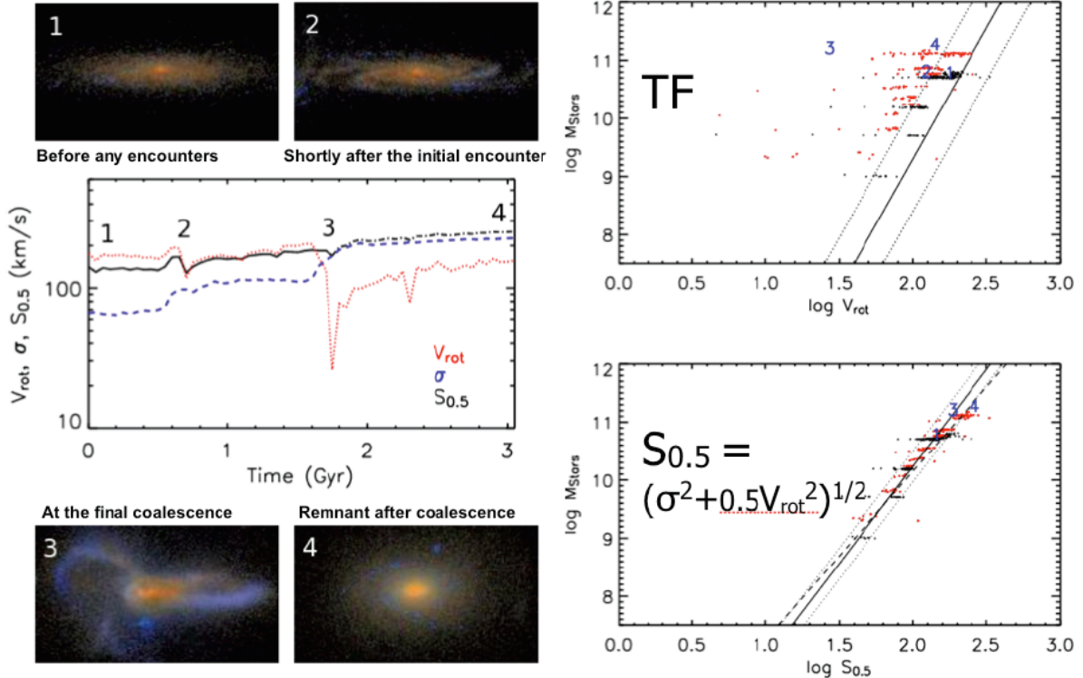
Figure 2: Left. Images of four merger stages (1 and 2 show one of the two merging galaxies, 3 and 4 show the merger and remnant). These are realistic images produced by our Sunrise code, including evolving stellar SEDs and radiative transfer through dust. The rotation velocity, velocity dispersion, and S_{0.5} are plotted vs. time, with the four merger stages indicated. Right. The upper panel is a Tully-Fisher-type plot of stellar mass vs. rotation velocity for our merger simulations observed including seeing effects, and the lower panel shows that adding \sigma and V_{\text{rot}} in quadrature greatly reduces the scatter as was found observationally. Black points represent individual galaxies, and red points represent cases where both galaxies are merged or lie in the same slit. The numbers indicate the four merger stages shown at left. (From Covington et al. 2009, submitted to MNRAS.)
