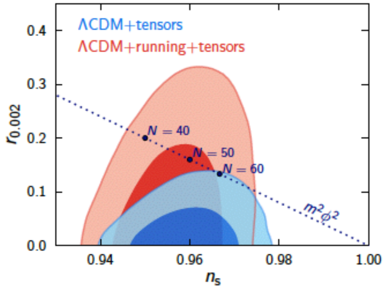
Planck Collaboration XVI (2013) Figure 23: Posterior distribution for n_s for the \Lambda CDM model with tensors (blue) compared to the posterior when a tensor component and running scalar spectral index are added to the model (red). The dotted line shows the relation between r and n_s for a V(\phi) inflaton potential where N is the number of inflationary e-foldings.
