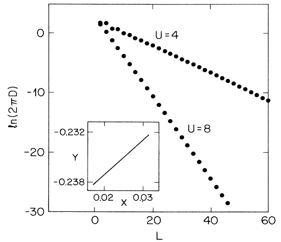
FIG. 1. \ln|2\pi D| as a function of system size for U = 4 (upper curve) and U = 8 (lower curve). \pi D is the dc spectral weight in units where e = \hbar = 1 . Inset: A plot of y = \ln[D(L)/D(40)]/(L-40) vs x = \ln[L/40]/(L-40) for L = 42-100 and U = 4 , displaying the asymptotic form y = -\xi^{-1} + \eta x . Here x = 4.06 and \eta = 0.45 .
