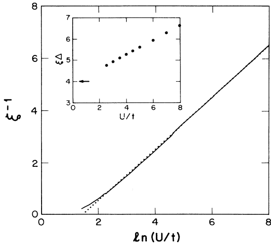
FIG. 2. The inverse of the localization length, \xi , vs \ln(U/t) . The analytic result \xi^{-1} = \ln(U/t) - 1.48 for U \gg t is shown as a dashed line. Note that \xi \rightarrow \infty as U \rightarrow 0 . Inset: \xi\Delta vs U/t , where \Delta is the Lieb-Wu charge gap. \xi\Delta appears to approach the mean-field result \xi\Delta/t = 4 (indicated by an arrow) as U \rightarrow 0 .
