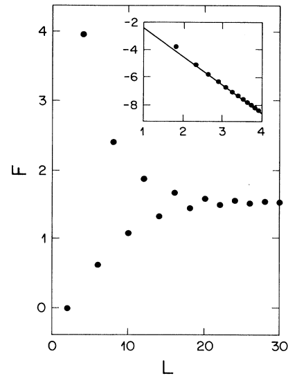
FIG. 3. Finite frequency spectral weight F = -(\pi/2L)\langle T \rangle - \pi D as a function of system size for U = 4 . Inset: Finite-size corrections to the total spectral weight displayed on a log-log plot for U = 10 , showing L^{-2} behavior.
