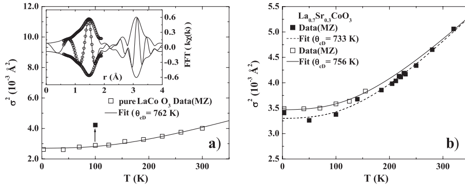
FIG. 2. (a) \sigma^2(T) for \text{LaCoO}_3 and the correlated Debye fit. The inset is an example of 4 K r -space data (solid line) and a fit to Co-O first peak (open circle); the Fourier transform (FT) range is 3.3\text{--}12.0 \text{ \AA}^{-1} with a Gaussian broadening of 0.3 \text{ \AA}^{-1} , and the r -space fit range is 1.1 to 1.7 \text{ \AA} . Note that we are fitting to the fast oscillating real and imaginary (not shown) parts of the FT. A good fit is obtained from 0.7\text{--}1.8 \text{ \AA} . (b) \sigma^2(T) for the \text{La}_{0.7}\text{Sr}_{0.3}\text{CoO}_3 JM samples. The solid squares represent the data from the first measurement, and open squares represent the data from the second measurement showing consistency between measurements taken a year apart; the dashed line is the correlated Debye fit for the first experiment data, while the solid line is the fit for the second experiment data. The solid symbol in (a) shows the increase in \sigma^2 if a 3-peak splitting occurs near 100 K.
