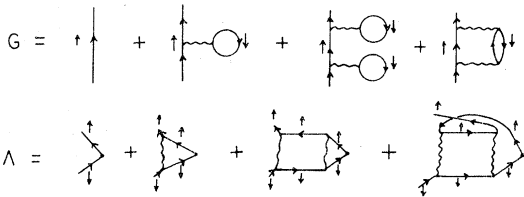
FIG. 1. All diagrams for G and \Lambda up to second order. The interaction is only between electrons of opposite spin.
