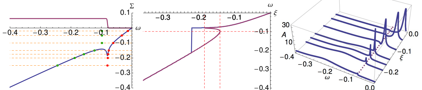
FIG. 2: Results for free electrons coupled to an Einstein phonon mode of frequency \omega_0 = .08 eV, with coupling strength \lambda = 0.5 , at T = 10 K. Right panel: The EDCs at several representative momenta, the variable \xi = v_f(k - k_F) = (1 + \lambda)V_L(k - k_F) here and in later figures. The dashed line indicates the phonon frequency, \omega = -\omega_0 . Each EDC has two well-defined features, a peak followed by a hump (separated by a sharp dip for low momentum EDCs). Middle panel: The MDC dispersion (magenta) has no jump while the EDC dispersion (blue) shows a jump. The two vertical dashed lines partition momentum space into three regions. The horizontal dashed line indicates the location of the hump in the EDCs in the first (low-momentum) region. In the first two regions, the EDC dispersion follows the MDC dispersion (closest to zero frequency), while in the third (high momentum) region, it stays pinned to the phonon frequency over a large range of momentum, until it discontinuously jumps back down to the MDC dispersion. Note that V_H = V_H^* . Left panel: \omega - \Re e \Sigma(\omega) and -\Im m \Sigma(\omega) vs. \omega . The horizontal dashed lines indicate the momenta associated with the corresponding EDCs in the right panel. The red dots indicate the locations of the peaks, and the green dots indicate the locations of the humps, as determined directly from each EDC.
