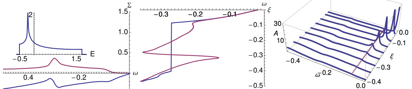
FIG. 5: We explore the effects of using the full frequency-dependence of the density of states in Eq. (SI-6), with \lambda = 0.84 and T = 115 K. Due to the functional form of the density of states (displayed as an inset in the left panel), the MDC dispersion acquires two additional branches which yield large frequency values. Below the low-energy kink momentum, the EDC dispersion follows the lowest-frequency branch of the MDC dispersion. Above the low-energy kink momentum, the EDC dispersion initially stays pinned to the phonon frequency, until it discontinuously jumps onto the highest-frequency branch of the MDC dispersion ( V_H = V_H^* ). A noticeable hump also develops at high-frequencies, in the corresponding EDCs.
