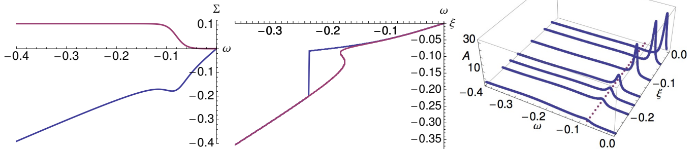
FIG. 4: We now use the experimentally relevant values of \lambda = 0.84 and T = 115 K. The curves retain the same qualitative features as in Fig. (2), which are less sharp in the present case due to the higher value of T .
