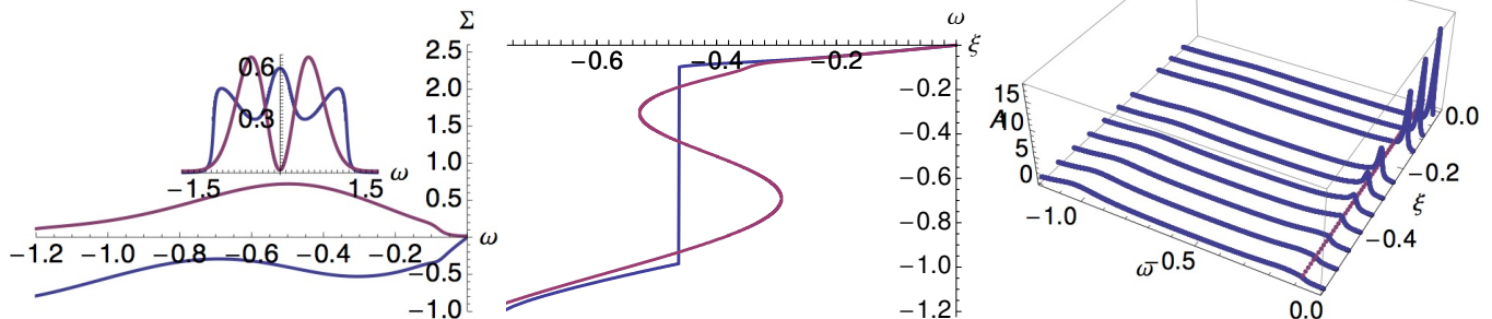
FIG. 6: We explore the effects of Fermi-liquid-like electron-electron correlations (Eq. (SI-8)), with \lambda = 0.84 and T = 115 K. Due to the functional form of the self-energy, \Sigma_{\text{el-el}}(\omega) (both -\Im\Sigma_{\text{el-el}}(\omega) and A_{\text{el-el,loc}}(\omega) ) are displayed as an inset in the left panel, the highest-frequency branch of the MDC dispersion yields very large values of the frequency. Below the low-energy kink momentum, the EDC dispersion initially stays pinned to the phonon frequency, until it discontinuously jumps onto the highest-frequency branch of the MDC dispersion ( V_H = V_H^* ). This is also reflected in the corresponding EDCs, which acquire a hump at high-frequencies.
