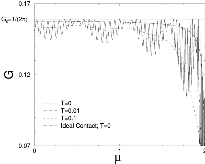
FIG. 2. Plot of conductance vs Fermi level, at three different temperatures ( T ), of a wire with a single impurity and imperfect contacts. The corresponding plot for perfect contacts at T=0 is also shown. The horizontal line is the ideal conductance G_0=1/(2\pi) (in units of e^2/\hbar ).
