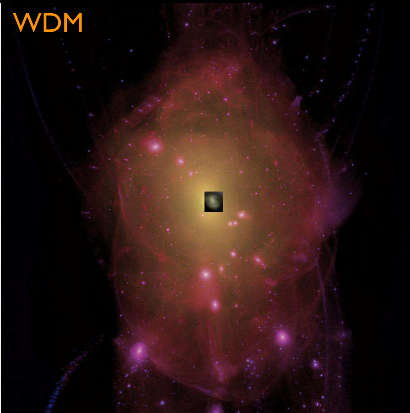
Lovell, Eke, Frenk, et al. 2012
