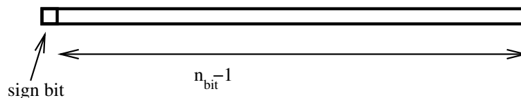
Representation of an integer
