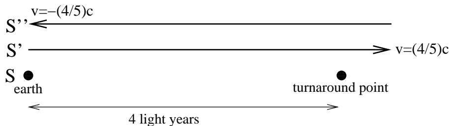
FIG. 1: In the twin “paradox”, one twin, Bob, stays on earth, an inertial frame which we will call S . At time zero, the other twin, Alice, gets on a moving walkway going with speed v = \frac{4}{5}c . This is also an inertial frame, which we call S' . She travels a distance 4 light years (as measured by Bob) and then jumps on to another moving walkway, moving in the opposite direction at the same speed, which carries her back to earth. This walkway is a third inertial frame, which we call S'' . We consider three events: event A when Alice leaves earth, event B when she turns round by jumping on to the returning walkway, and event C when she arrives back on earth.
